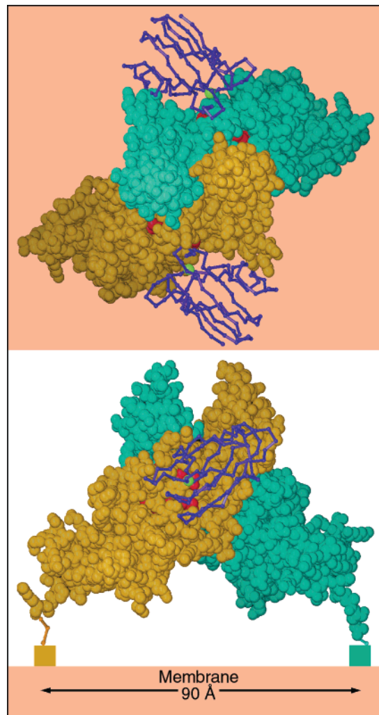
FIGURE 6: Dimer-like noncrystallographic symmetry observed in the crystal of C. reinhardtii cytochrome f , and interaction with plastocyanin modeled from ref 50. Above is a top view, looking down the 2-fold axis of symmetry. Below is a side view, looking parallel to a hypothetical membrane plane (orange) constructed perpendicular to the 2-fold axis. The blue and yellow space-filling models are monomers A and B from the crystal of C. reinhardtii cytochrome f , respectively. The hemes are shown as red space-filling models. The rectangles below the C termini in the lower panel represent the luminal ends of the transmembrane helices. The magenta backbone drawings are C. reinhardtii plastocyanin (66) oriented as in the NMR structure of the plastocyanin–cytochrome f complex (2PCF), oriented with the operators that best superimpose cytochrome f of that structure on each monomer of the C. reinhardtii dimer. The copper atom of plastocyanin is shown as a green sphere. The interactions between these two monomers in the crystal may be similar to those involved in stabilizing a physiological dimer in vivo (see the text). In this figure, monomer B is taken directly from structure 1CFM; monomer A is transformed by crystallographic symmetry operator [\frac{1}{2} + x, \frac{1}{2} - y, 1 - z] because the chosen asymmetric unit does not include this dimer. For positioning plastocyanin, the rotation translation operator giving the best superposition of C. reinhardtii plastocyanin in entry 1PLT with poplar plastocyanin in entry 2PCF (over residues 5–45 and 65–95) was multiplied on the left by the operator giving the best superposition of turnip cytochrome f with C. reinhardtii cytochrome f monomers A and B oriented as described above (superimposing residues 1–4, 27–30, 45–52, 68–76, 111–117, and 142–159 of turnip with the same residues in C. reinhardtii and residues 234–238 of turnip with residues 235–239 of C. reinhardtii ).
